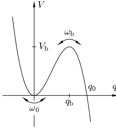
Fig. 4.2: Cubic potential as defined by (4.160).
